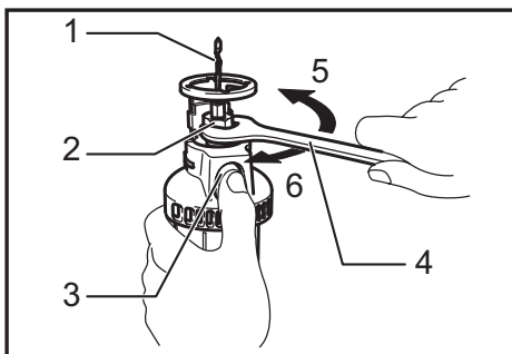
► 1. Bit 2. Collet nut 3. Shaft lock 4. Wrench 5. Loosen 6. Tighten
