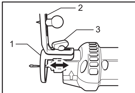
► 1. Shoe 2. Circular guide 3. Thumb screw
